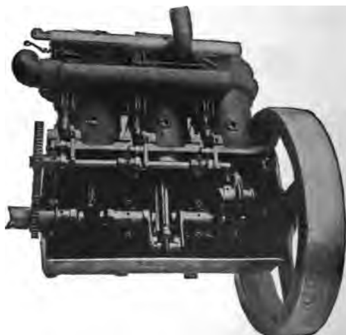
FIG. 208.—The Duryea Three-Cylinder Gasoline Vehicle Engine, with half the crank case sheathing removed, showing cranks, crank shaft, cam shaft, and working parts. The three cylinders have common supply and exhaust tubes; the charge is controlled by a single throttling link, shown at the top, and the igniting circuit has three bridges for the three cylinders. Cranks, as indicated, are at 120 degs.
